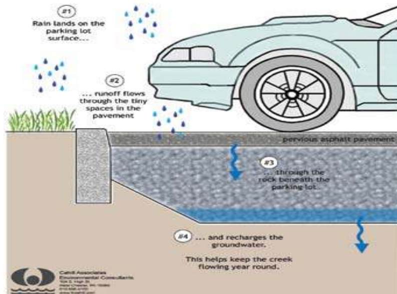
Figure 1 Pervious Pavement with infiltration schematic
