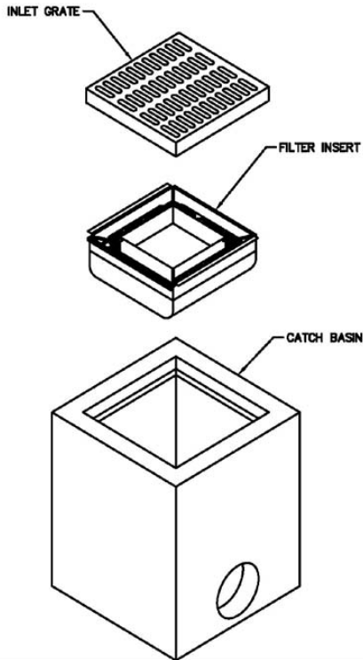
Figure 2 Tray type insert Source: Pennsylvania Stormwater BMP Manual, 2004
