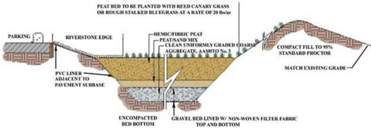
PARKING LOT VEGETATED PEAT FILTER EXAMPLE (CA)
