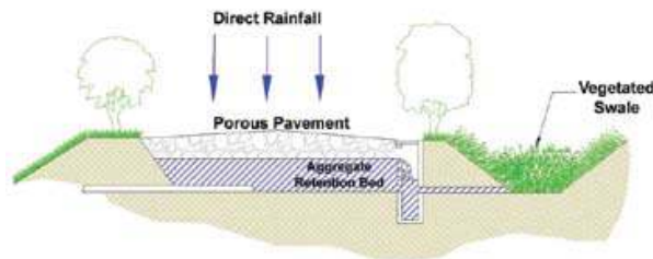
Figure 3 Slow discharge from porous pavement bed to vegetated swale Source: Pennsylvania Stormwater BMP Manual 2006
