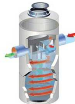
Figure 5 Example of Hydrodynamic Devices Sources: Stormwater Solutions (top) and Terre Hill Stormwater Solutions (bottom)
