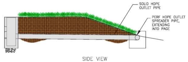
Figure 3 A level spreader with a perforated pipe
